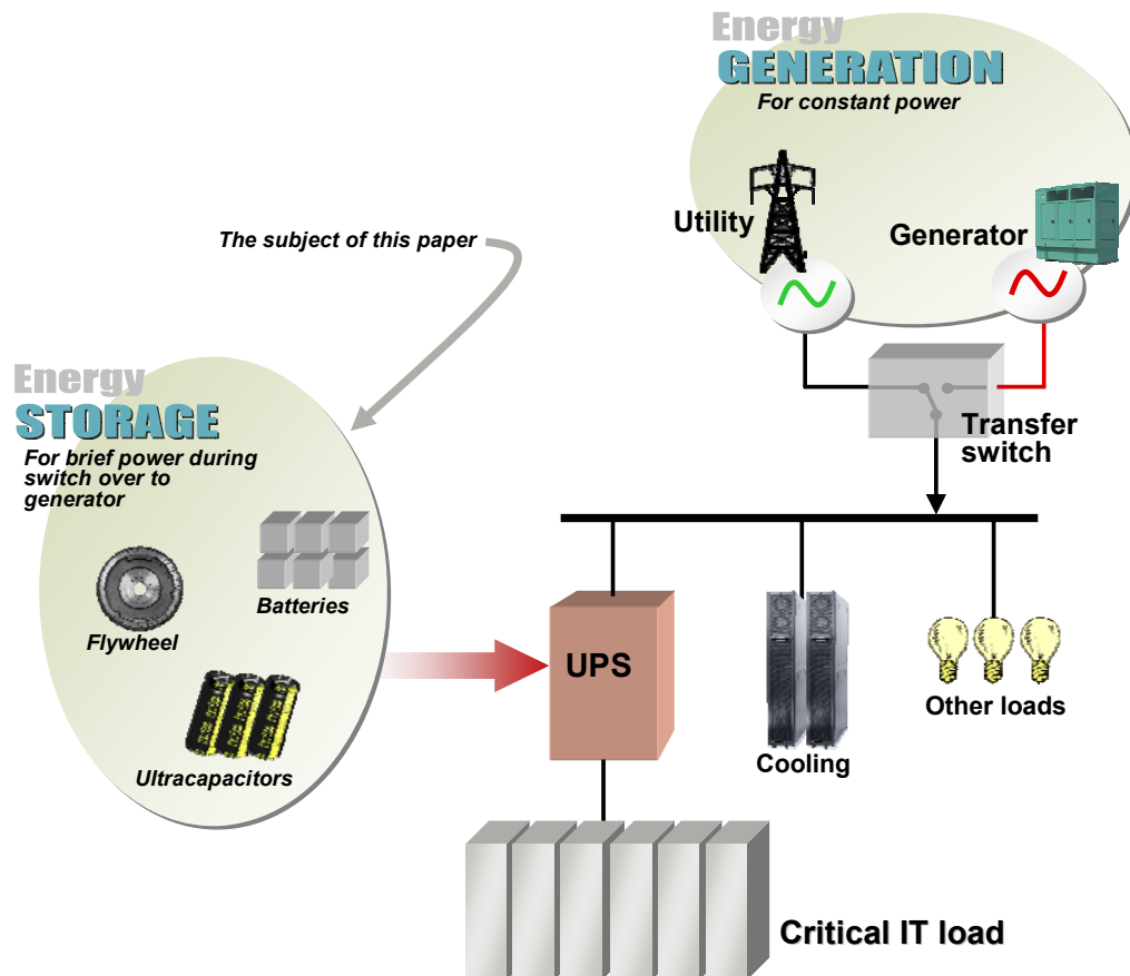
Figure 1 – Energy storage in the context of the data center power path
