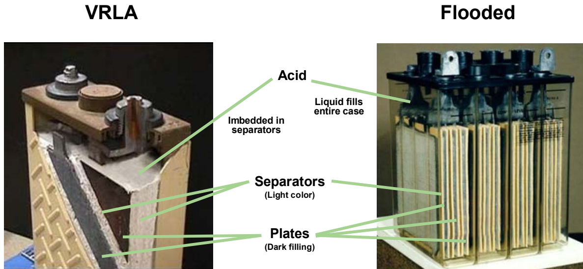
Figure 4 – Typical lead-acid battery
