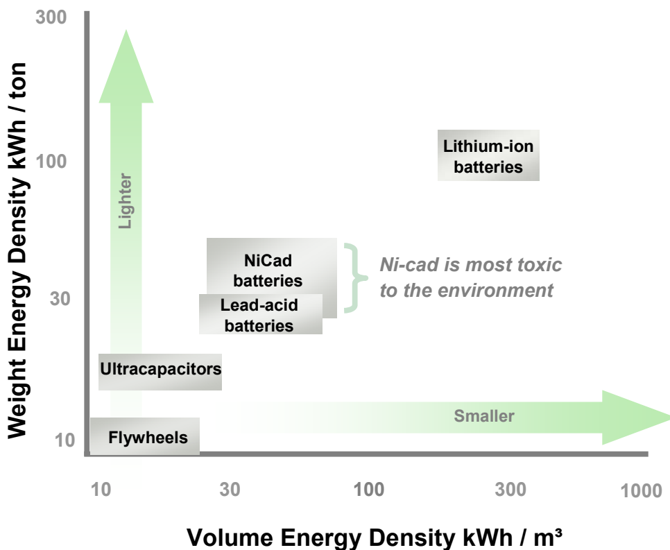
Figure 3 – Technology size and weight comparisons 2
