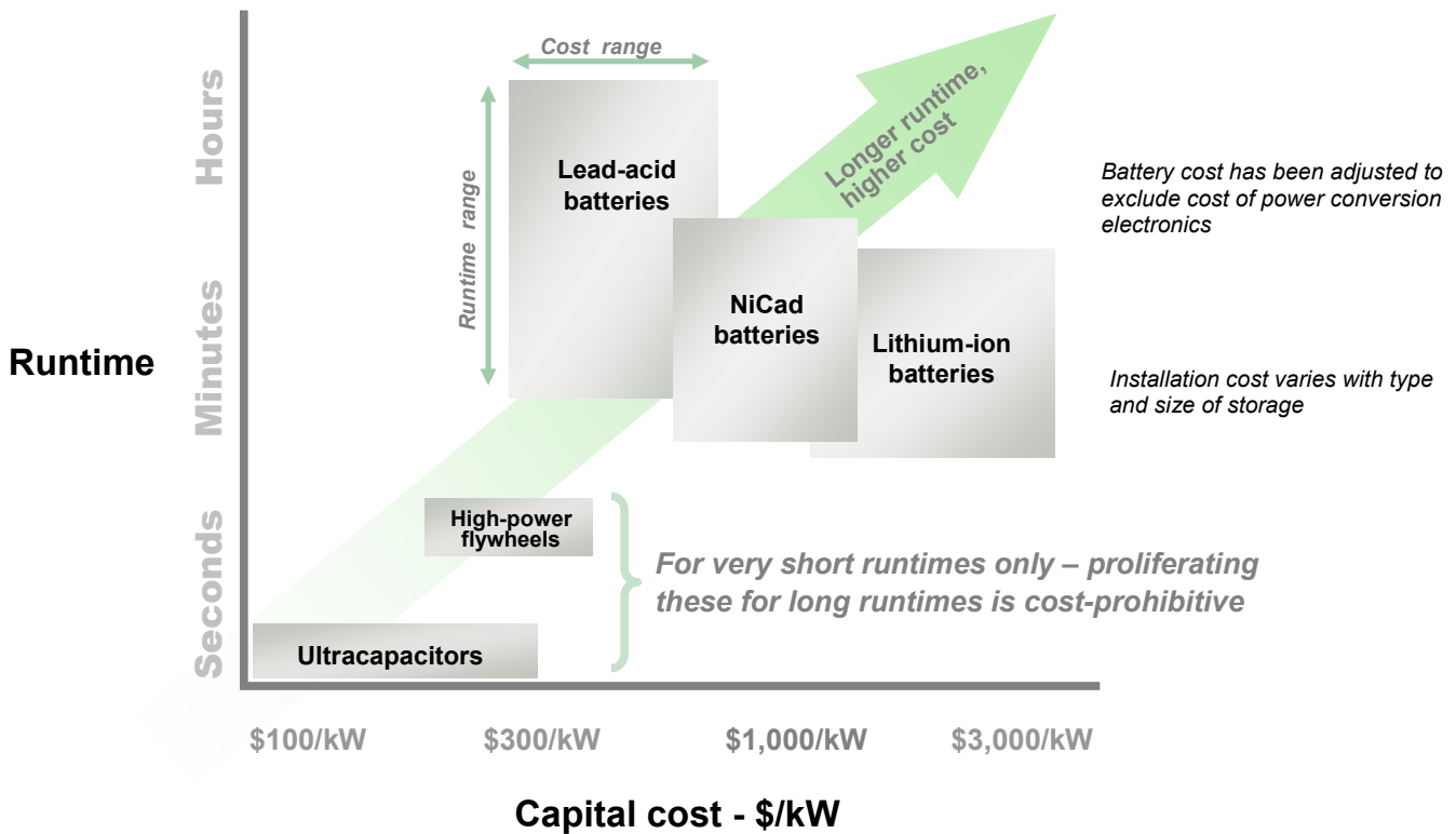
Figure 2 – Capital cost vs. runtime for energy storage methods 1
