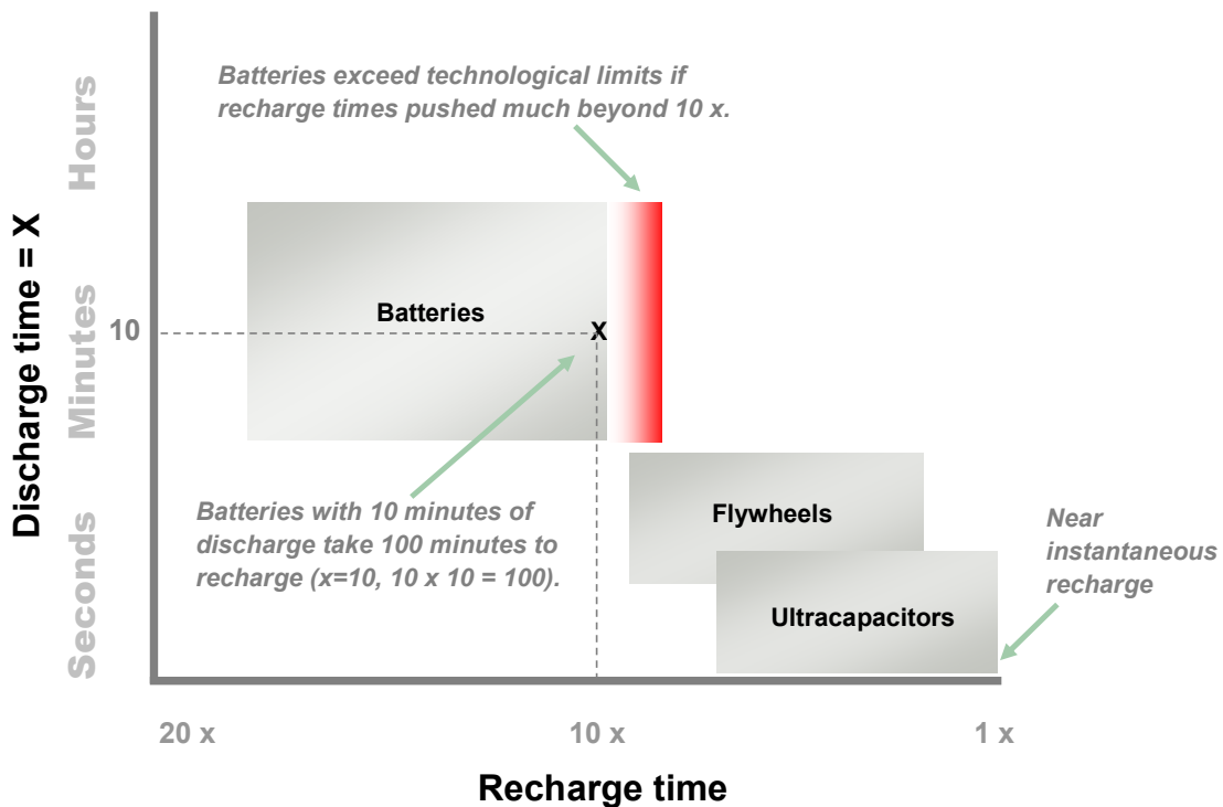
Figure 5 – Comparison of energy storage technology discharge / recharge times
